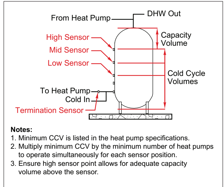
Figure 9: Single-pass, Multiple Heat Pumps with Central Controller
