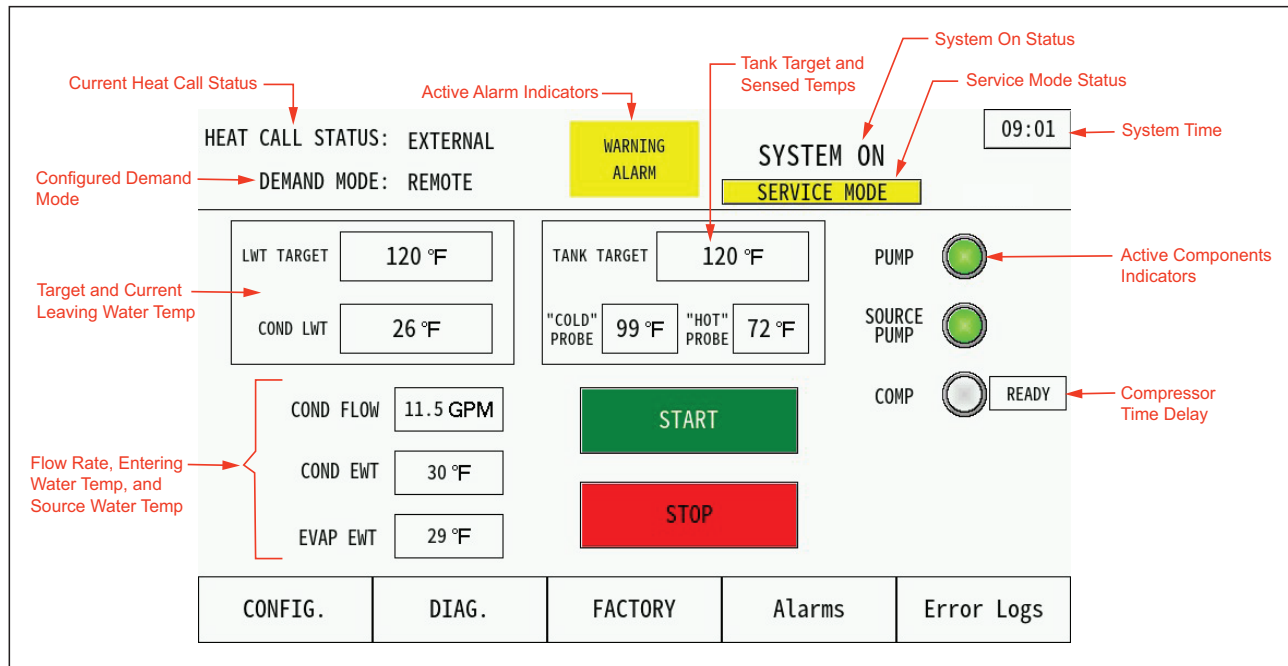
Diagram 11: Diagnostic Interface Page
