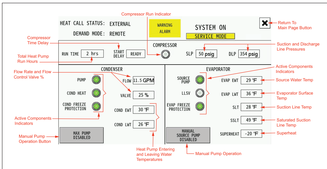
Diagram 11: Diagnostic Interface Page
