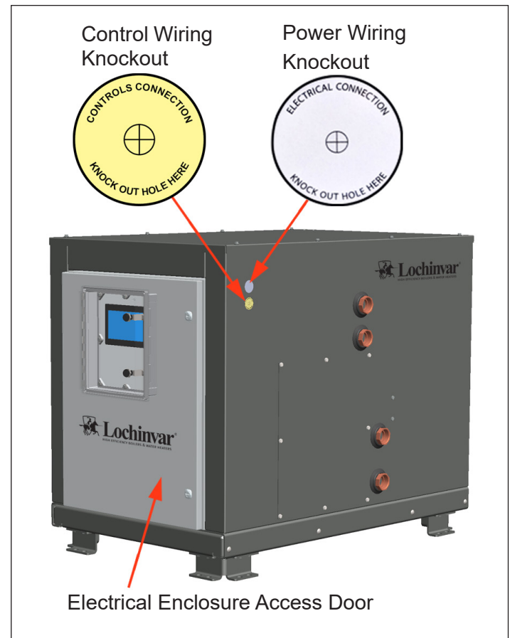
Figure 7: Electrical Knockouts Locations
