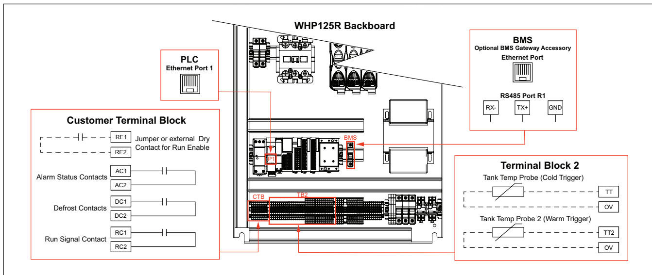
Diagram 5: WHP125R Control Wiring
