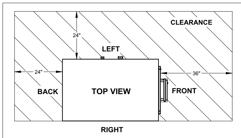
Figure 1: WHP125R Model Clearances
