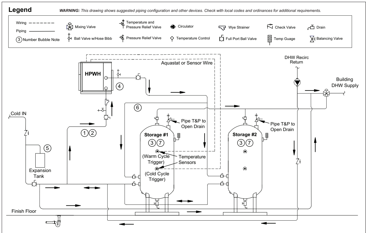
Diagram 3: Multi-pass Piping Concept
