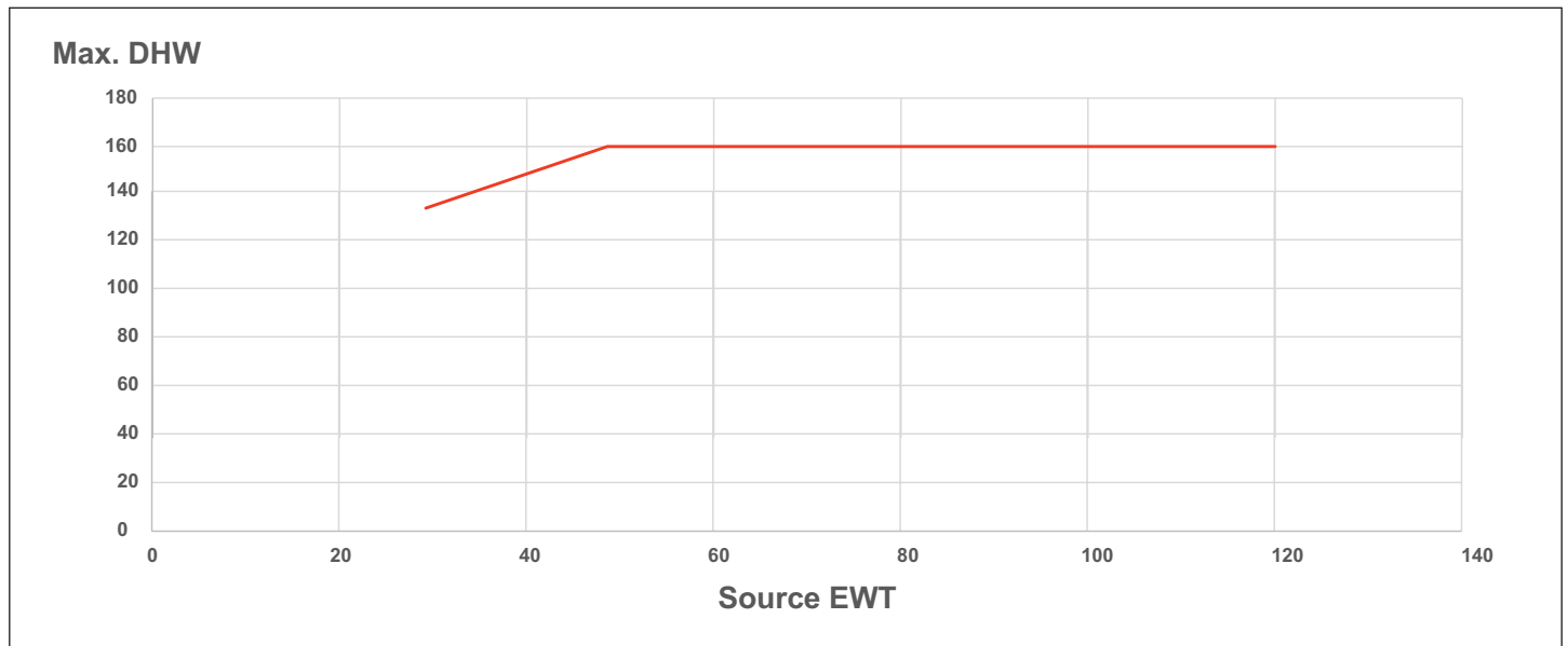
Diagram 1: Source EWT - Maximum DHW LWT
