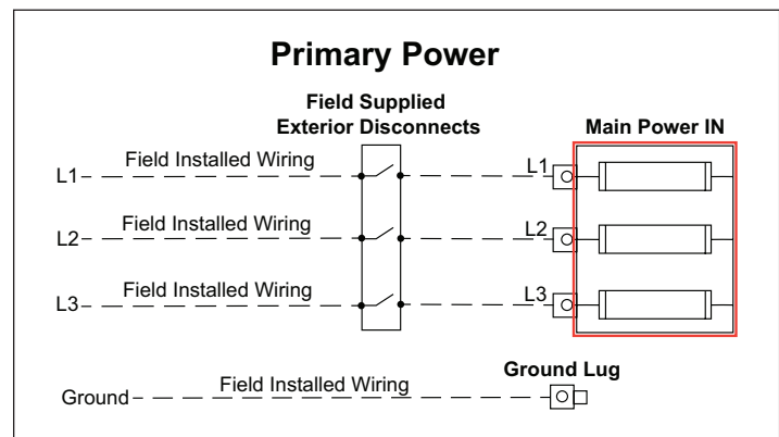
Diagram 4: Power Wire Connections
