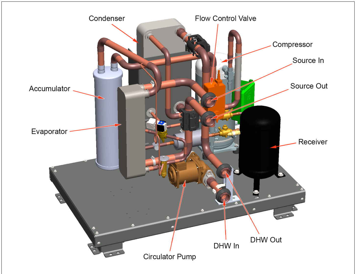
Figure 2: WHP125R Model
